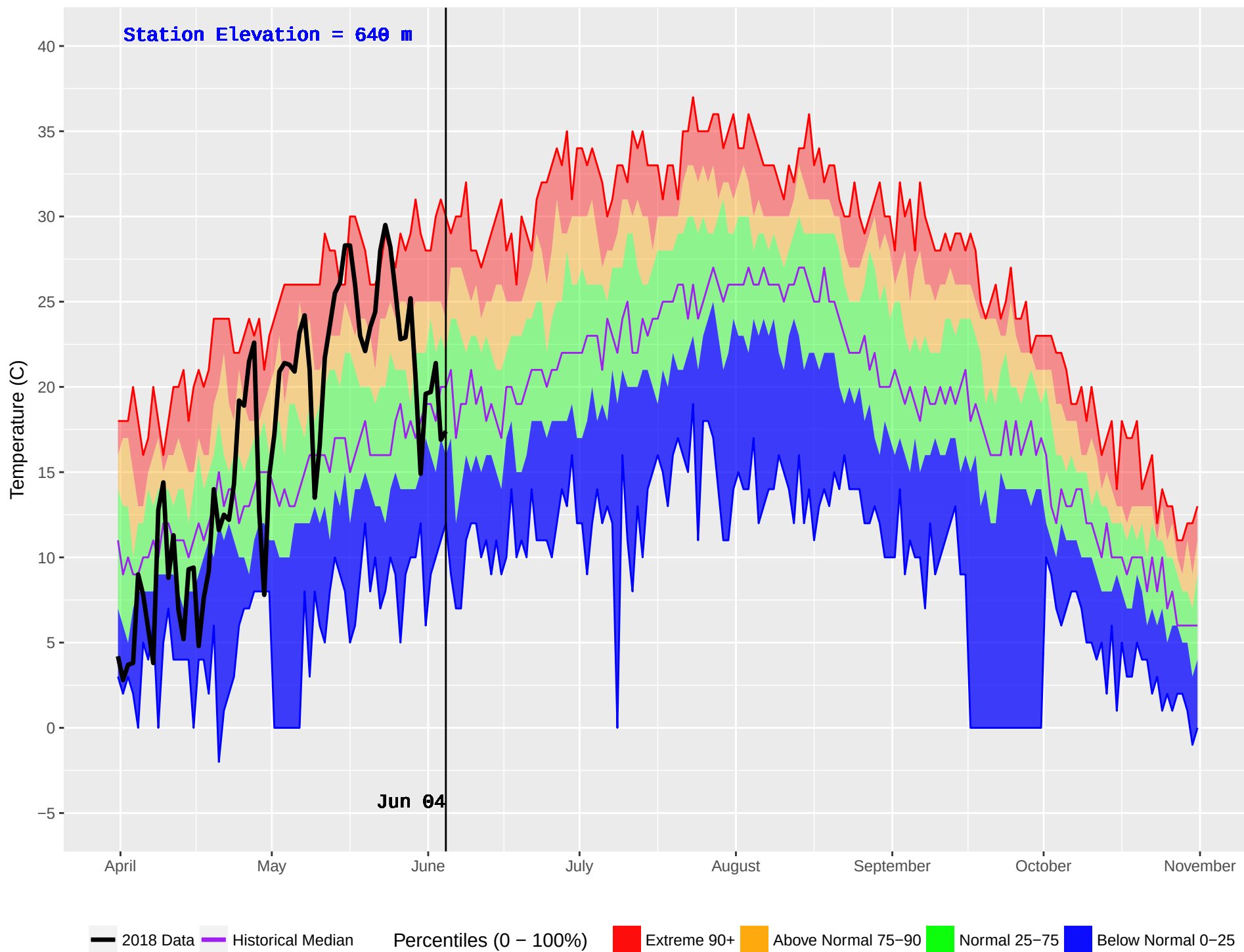
TURTLE (286) : Historical (1977–2016) and Current (2018) Noon Temperature
