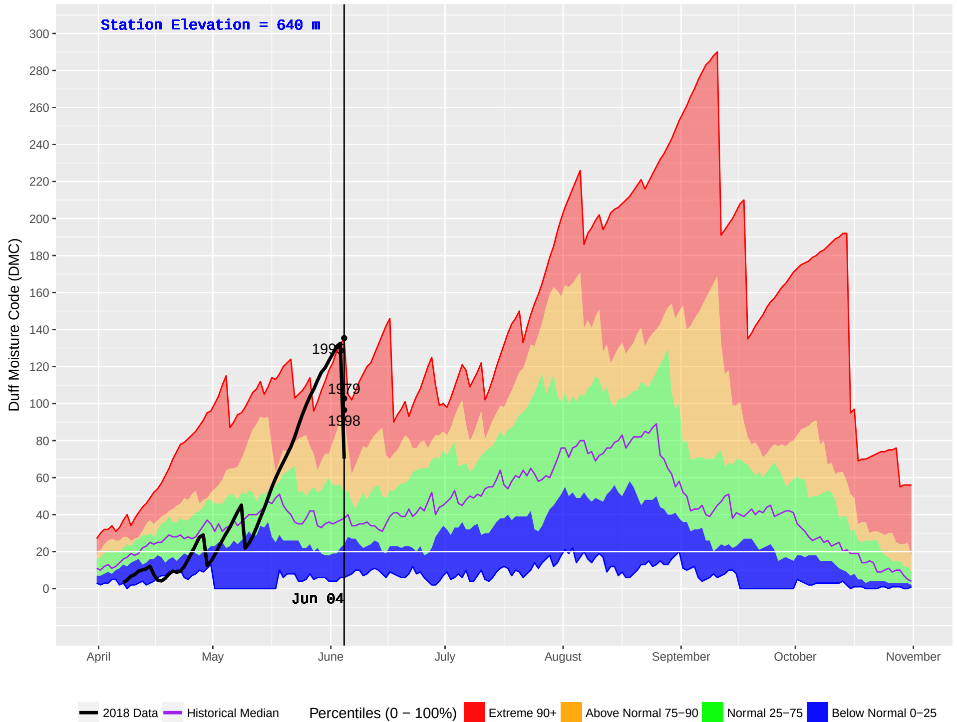
TURTLE (286) : Historical (1977–2016) and Current (2018) Noon Duff Moisture Code (DMC)
